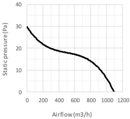
VMA-30C4S
