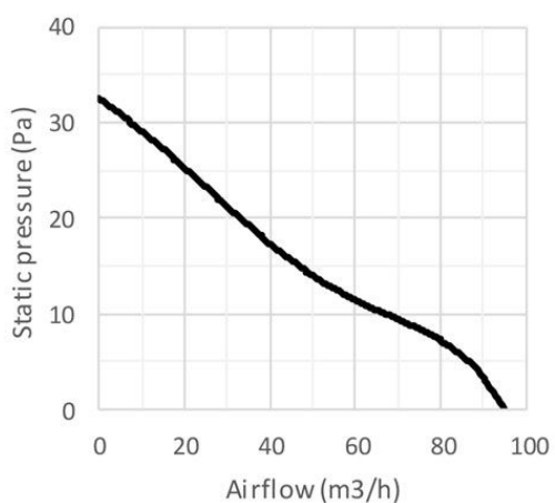
VMA-10S2S
