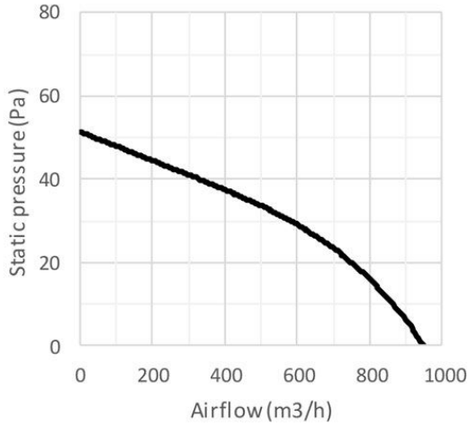
VMA-25C2S
