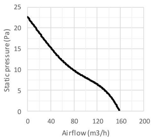
VMA-12S2S
