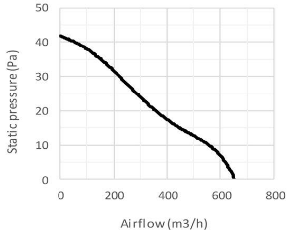
VMA-25C4S
