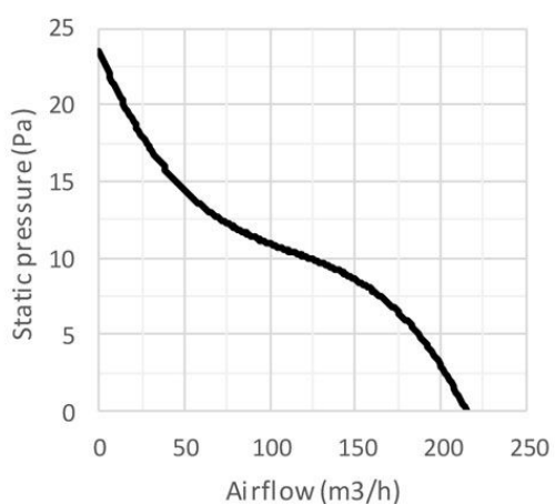
VMA-15S2S
