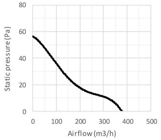
VMA-20C4S
