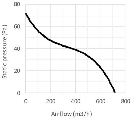
VMA-20C2S
