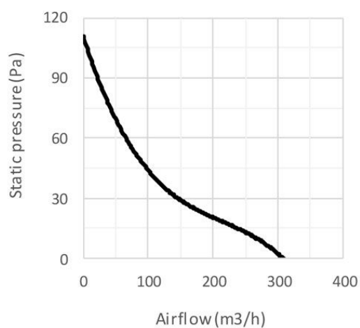
VMA-15C2S
